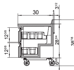
Interior Dimensions
