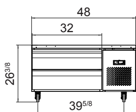
MGF8460GR
