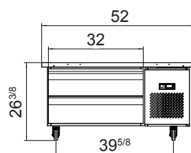
MGF8461GR
