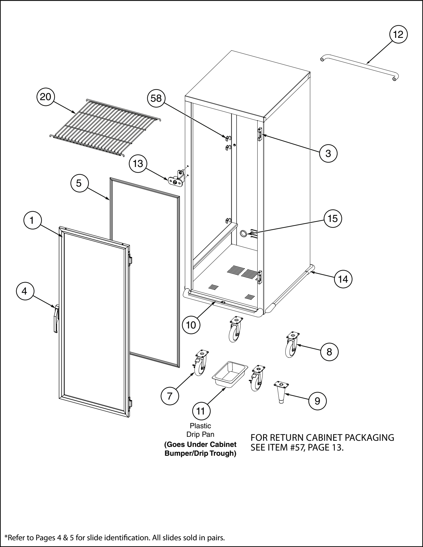
C5 1 Series Cabinet Replacement Parts Diagram (Both 120V & 220-240V)
